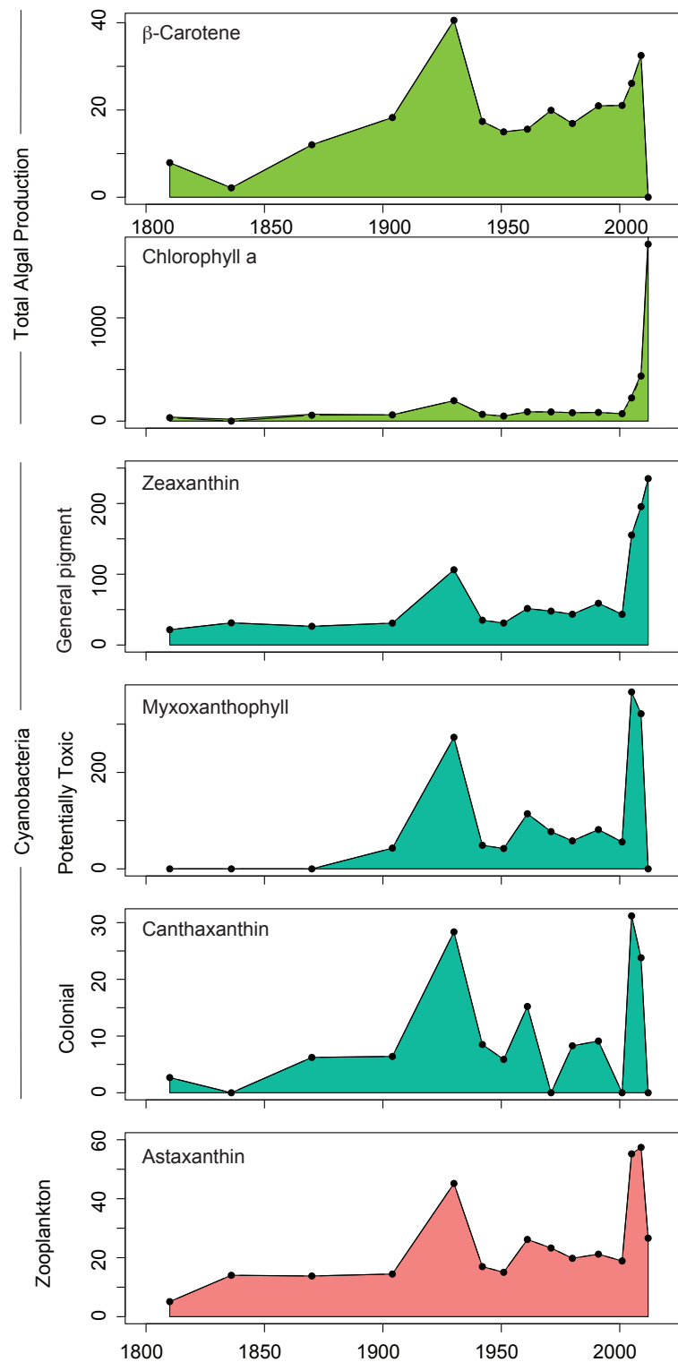
Figure 7: The sediment algal pigments present in Spring Lake. The group of algae associated with each pigment is shown along the y-axis. In addition to algal pigments, zoo-plankton pigment is present in large abundance.
