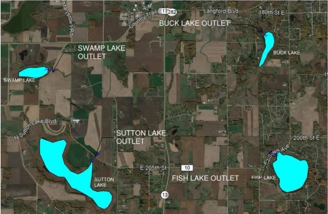
Figure 5.16. Upper Watershed Lakes Controlled Outlet Storage concept.
